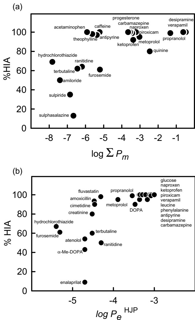
Figure 7.67 Human intestinal absorption compared to (a) pI\text{ON} 's double-sink sum- P_e PAMPA GIT model and (b) human jejunal permeabilities [56].
