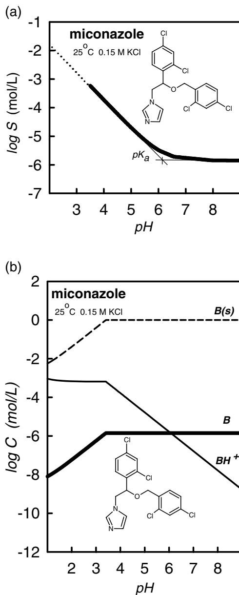
Figure 6.2 Solubility-pH profile (a) and a log-log speciation plot (b) for a weak base (miconazole, pK_a 6.07, \log S_0 -5.85 [pION]). [Avdeef, A., Curr. Topics Med. Chem. , 1 , 277–351 (2001). Reproduced with permission from Bentham Science Publishers, Ltd.]
